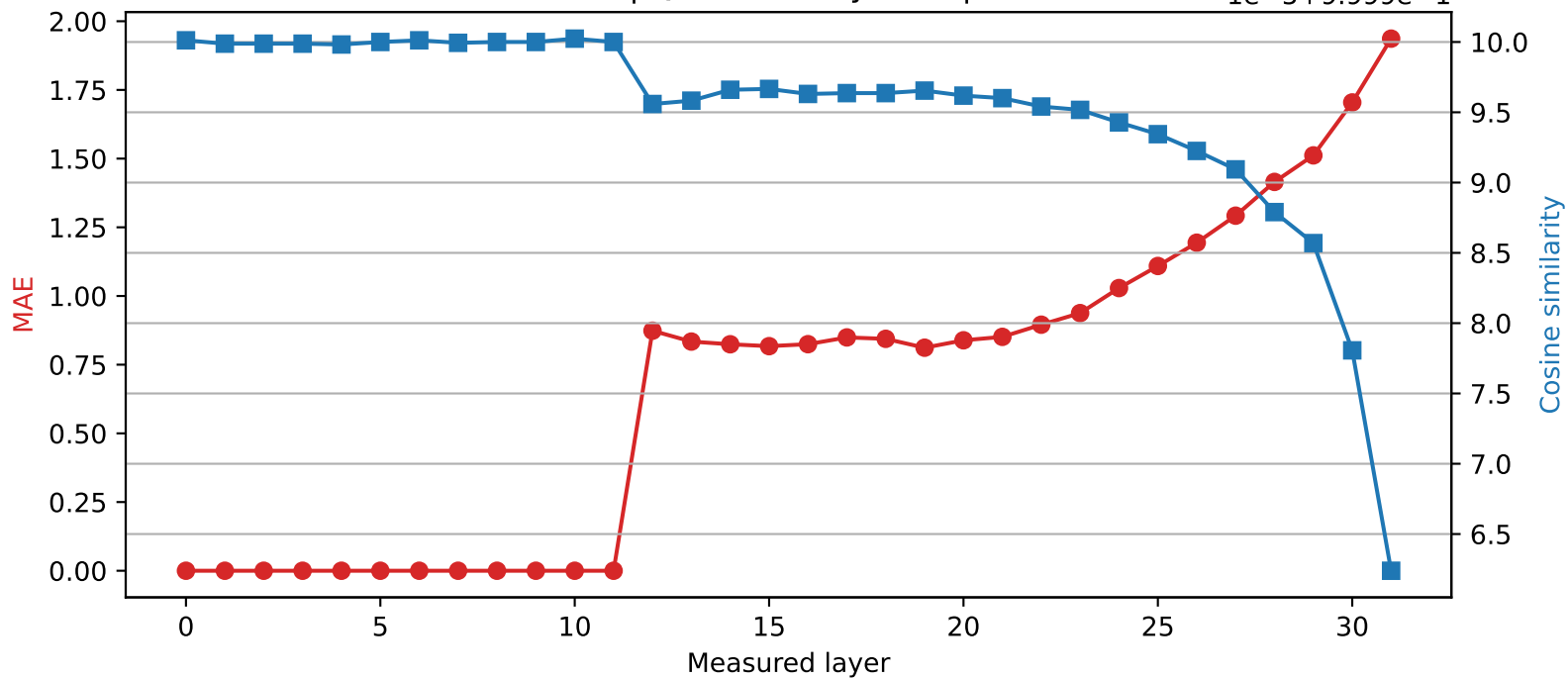
SmolLM2-360M | Quantized layer 11 | float64 → int2 1e-5+9.999e-1
