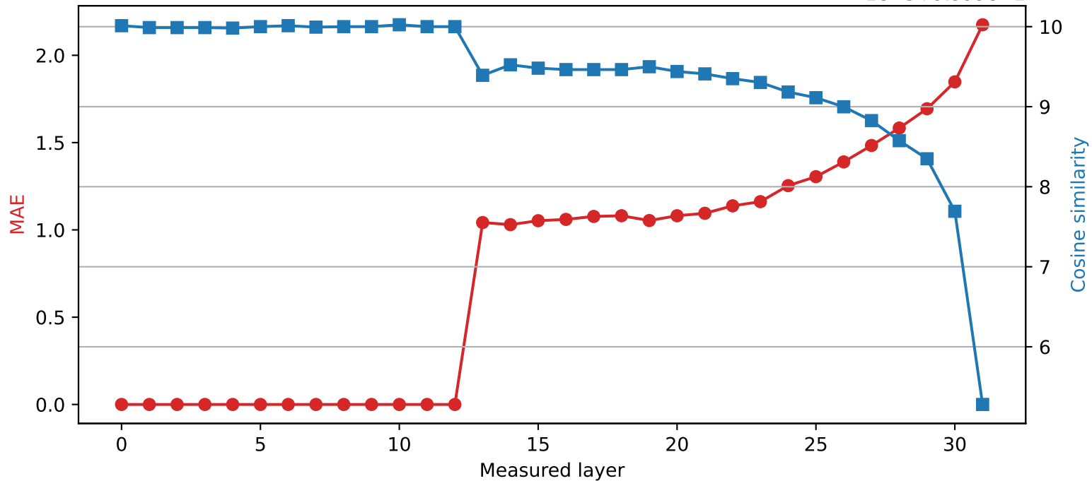
SmolLM2-360M | Quantized layer 12 | float64 → int2 1e-5+9.999e-1
