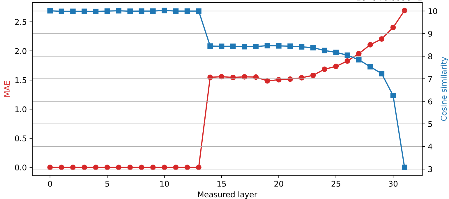
SmolLM2-360M | Quantized layer 13 | float64 → int2 1e-5+9.999e-1
