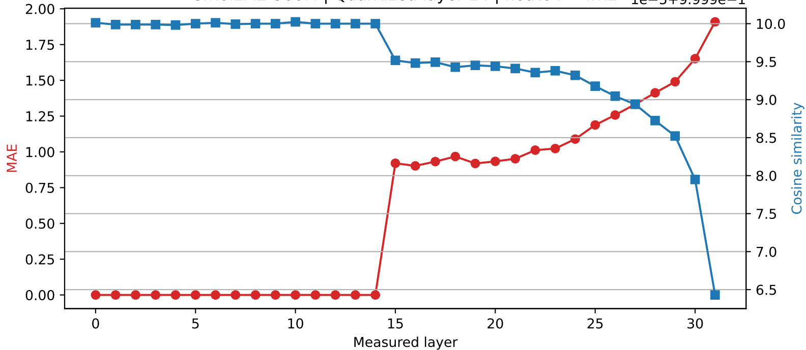
SmolLM2-360M | Quantized layer 14 | float64 → int2 1e-5+9.999e-1
