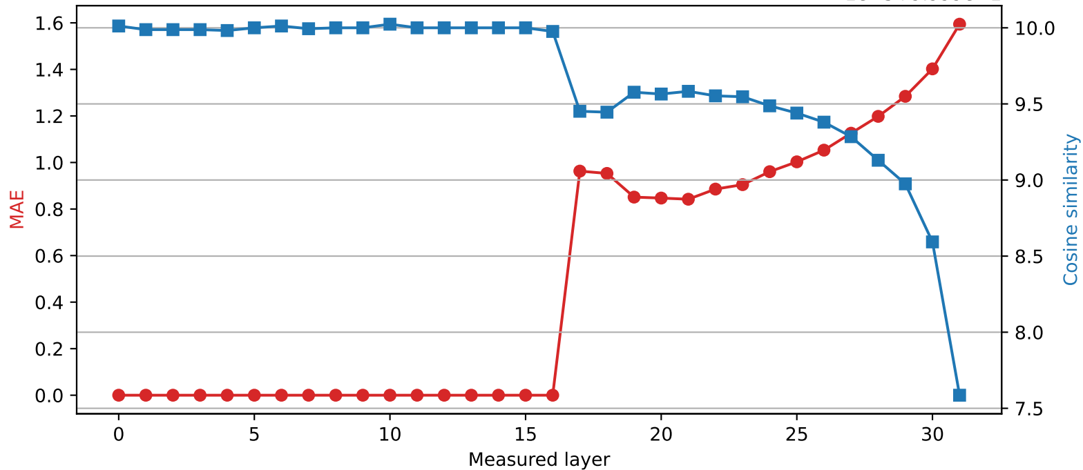
SmolLM2-360M | Quantized layer 16 | float64 \rightarrow int2 1e-5+9.999e-1
