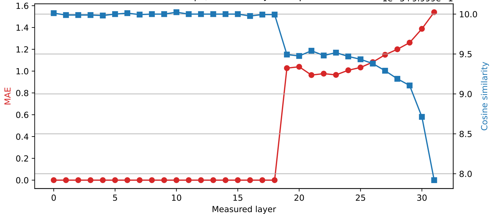
SmolLM2-360M | Quantized layer 18 | float64 \rightarrow int2 1e-5+9.999e-1
