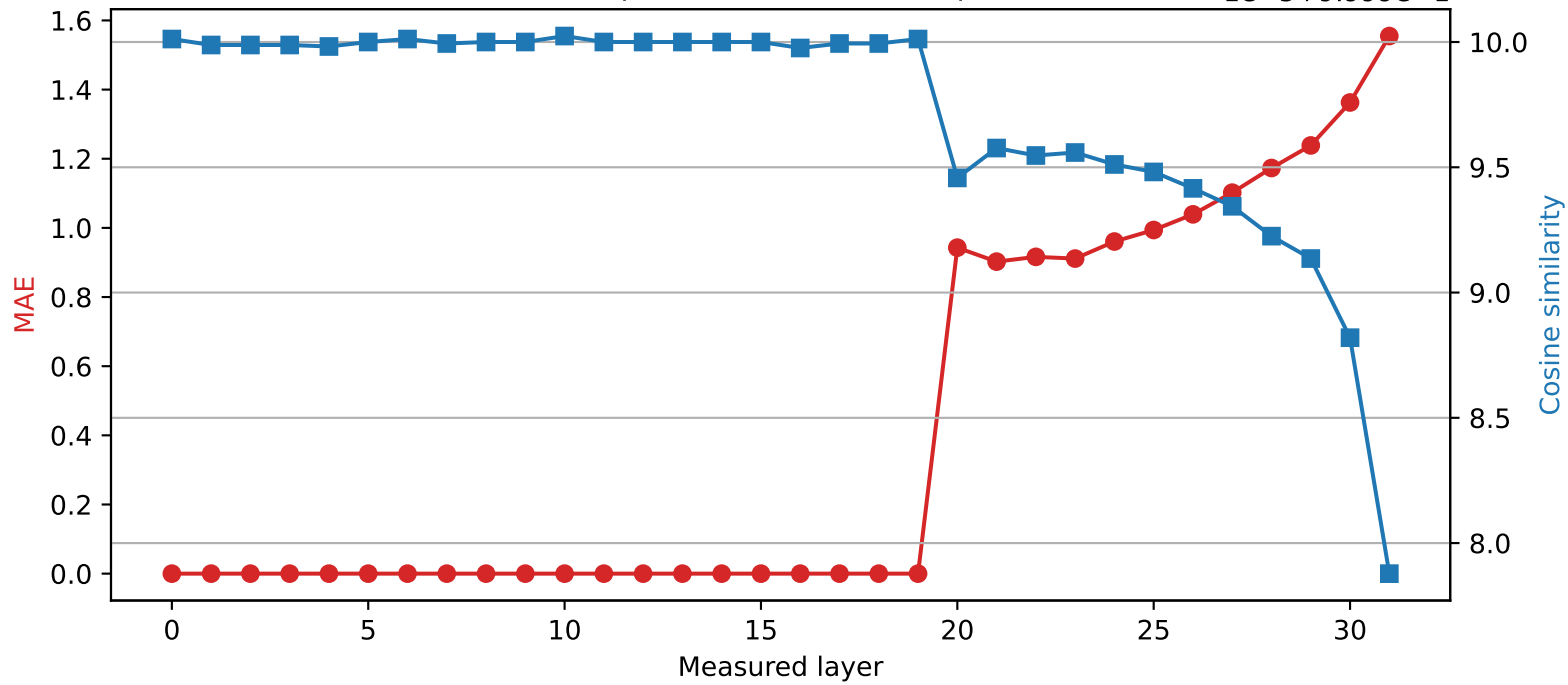
SmolLM2-360M | Quantized layer 19 | float64 \rightarrow int2 1e-5+9.999e-1
