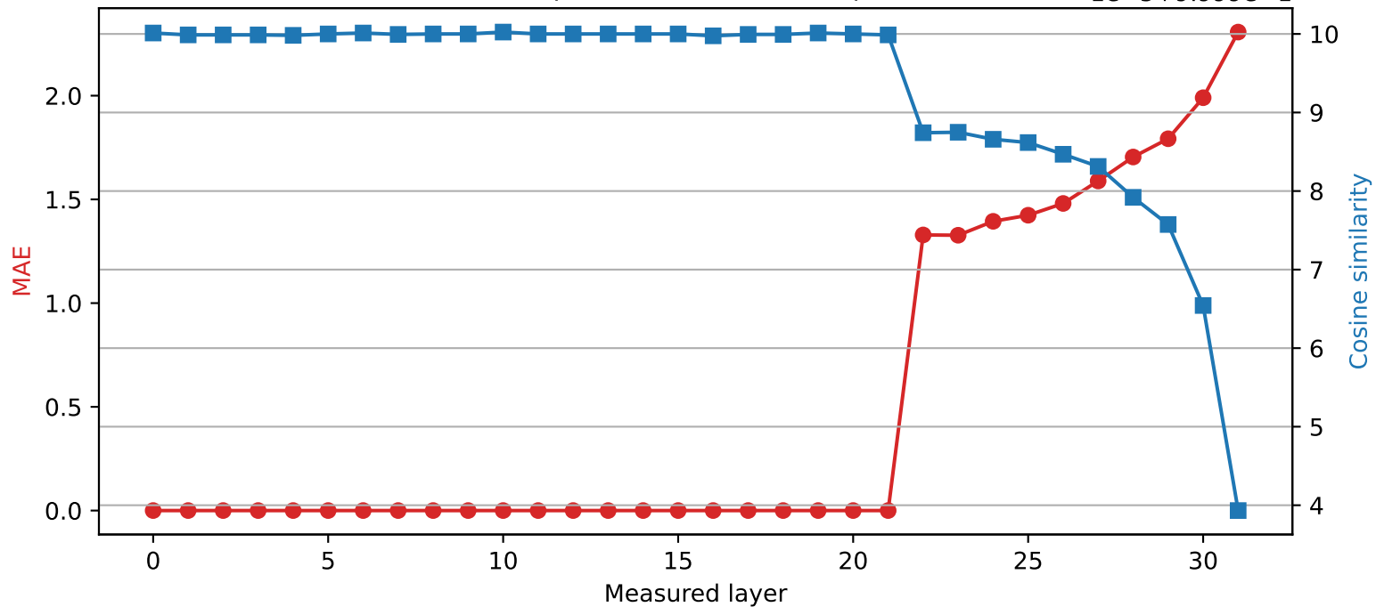
SmolLM2-360M | Quantized layer 21 | float64 \rightarrow int2 1e-5+9.999e-1
