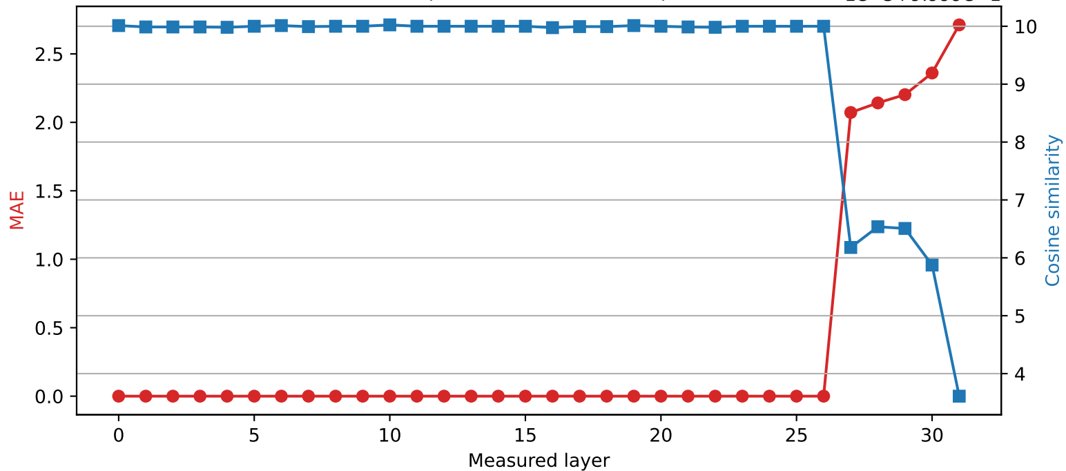
SmolLM2-360M | Quantized layer 26 | float64 → int2
