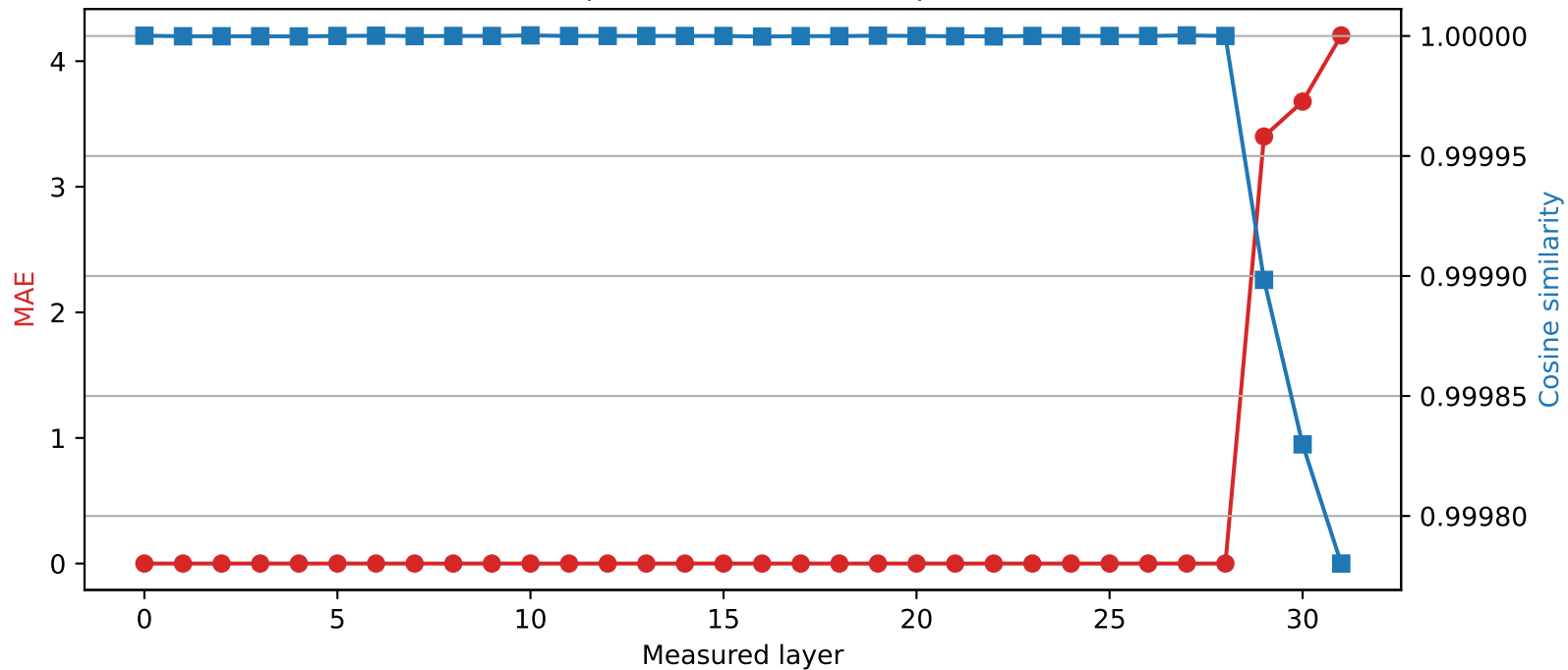
SmolLM2-360M | Quantized layer 28 | float64 → int2
