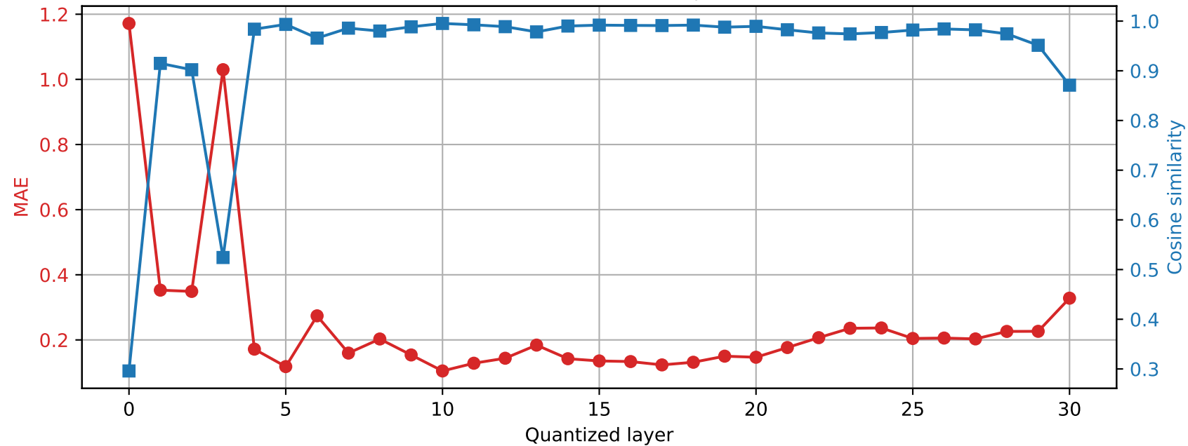
SmolLM2-360M | Prompt 1 Final RMSNorm output damage | float64 → int2
