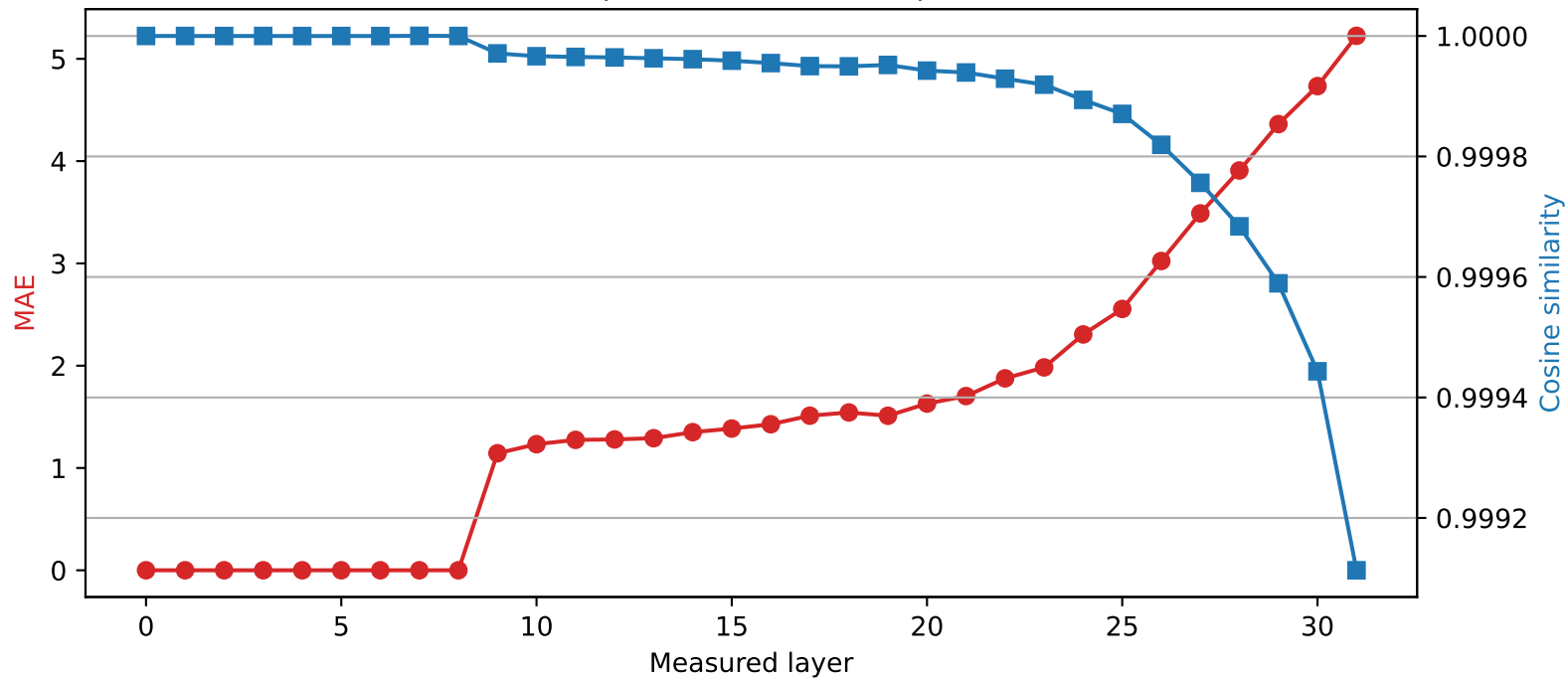
SmolLM2-360M | Quantized layer 8 | float64 \rightarrow int2
