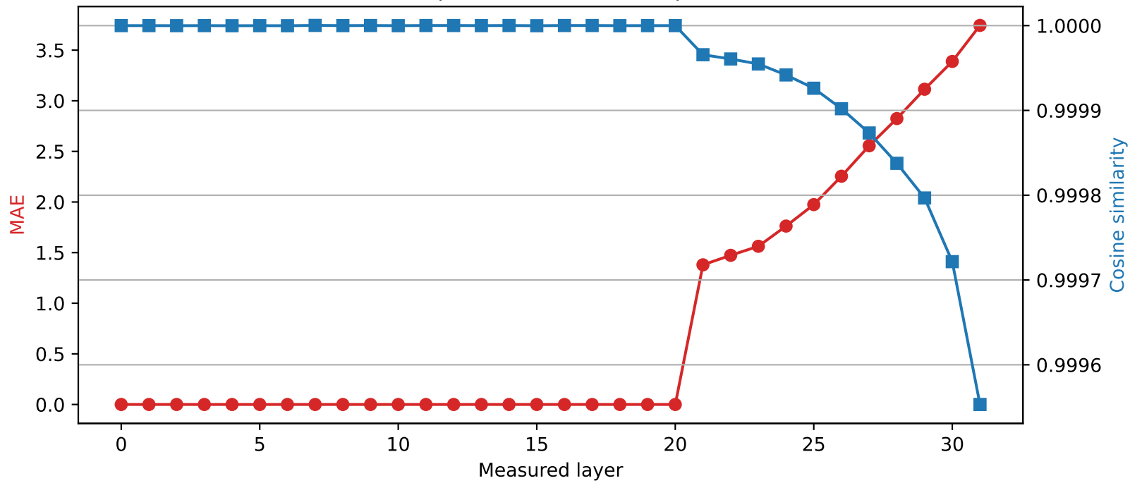
SmolLM2-360M | Quantized layer 20 | float64 \rightarrow int2
