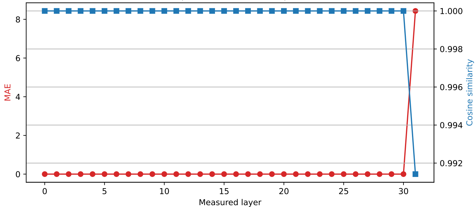
SmolLM2-360M | Quantized layer 30 | float64 → int2
