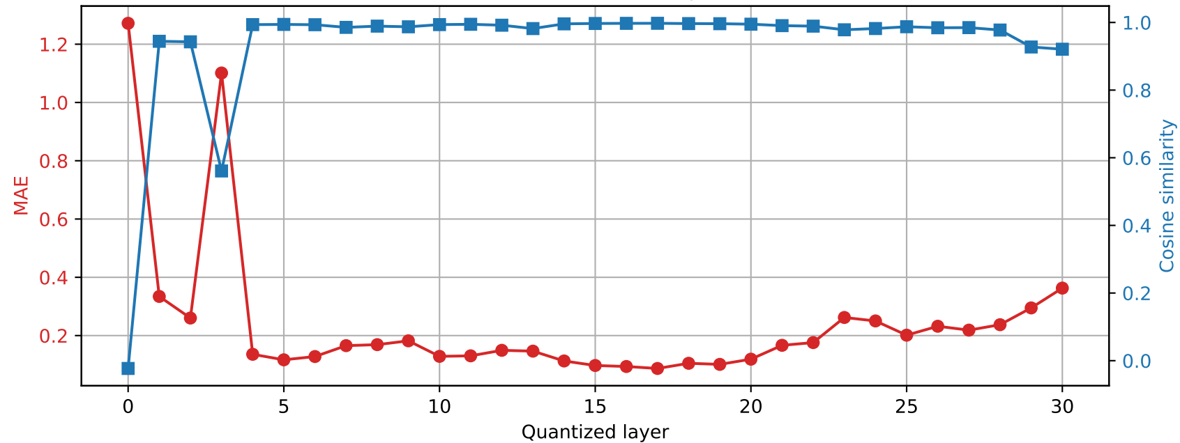
SmolLM2-360M | Prompt 2 Final RMSNorm output damage | float64 \rightarrow int2
