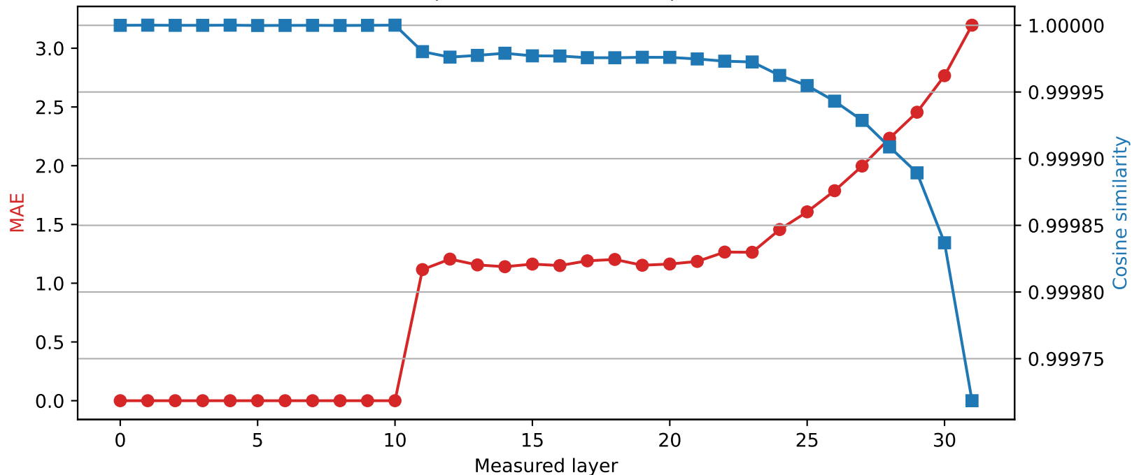
SmolLM2-360M | Quantized layer 10 | float64 → int2
