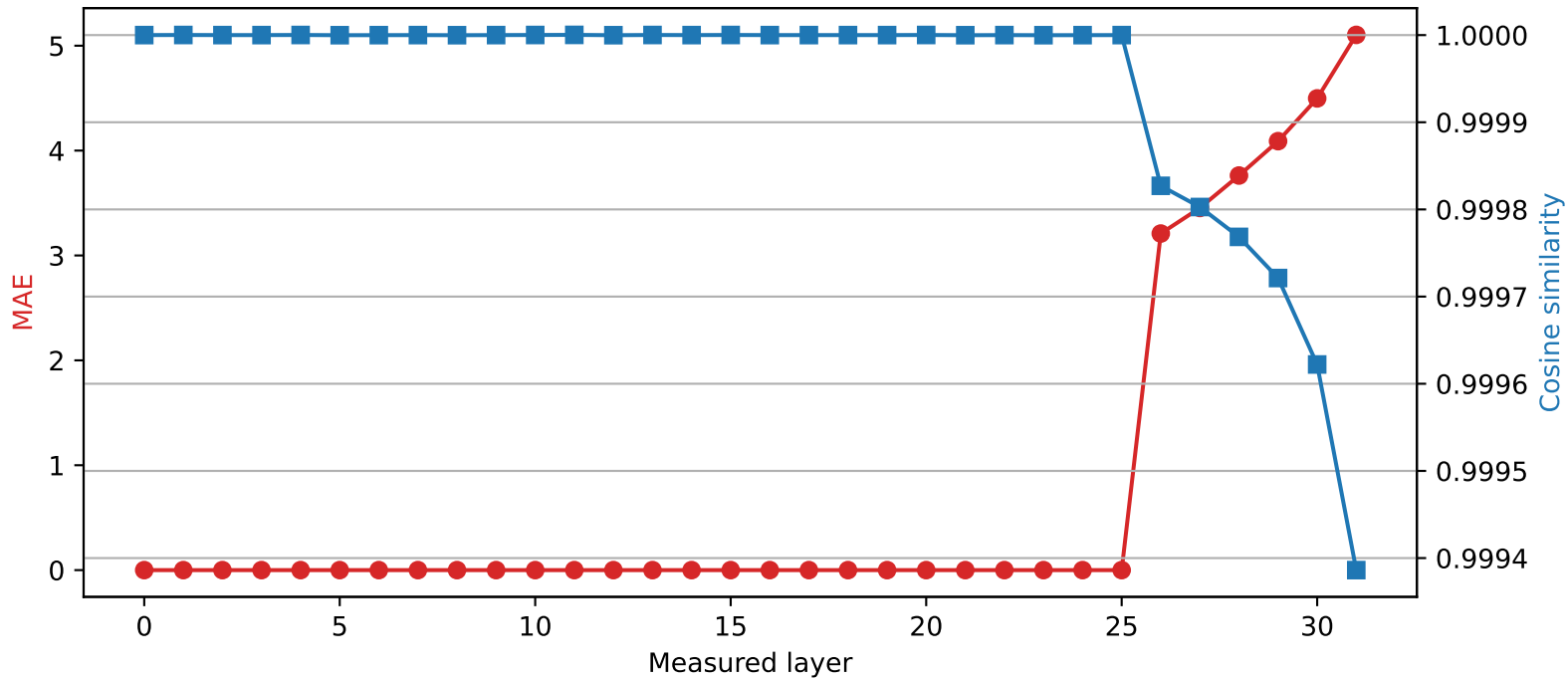
SmolLM2-360M | Quantized layer 25 | float64 → int2
