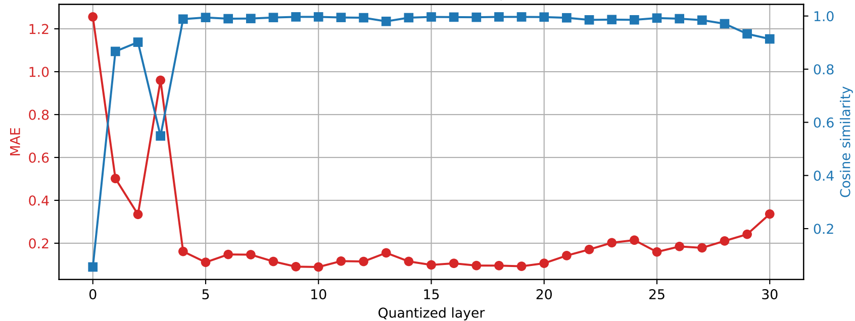
SmolLM2-360M | Prompt 3 Final RMSNorm output damage | float64 \rightarrow int2
