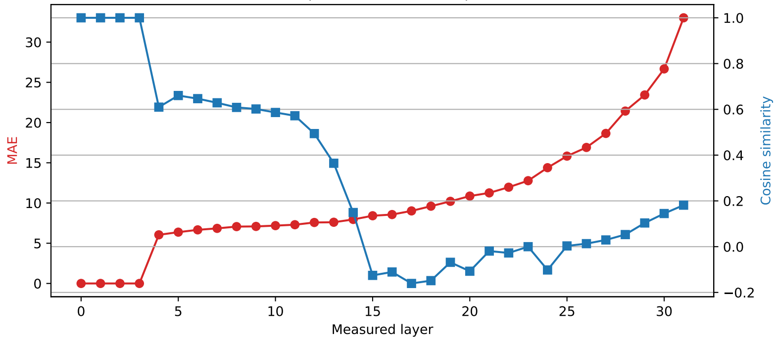
SmolLM2-360M | Quantized layer 3 | float64 → int2
