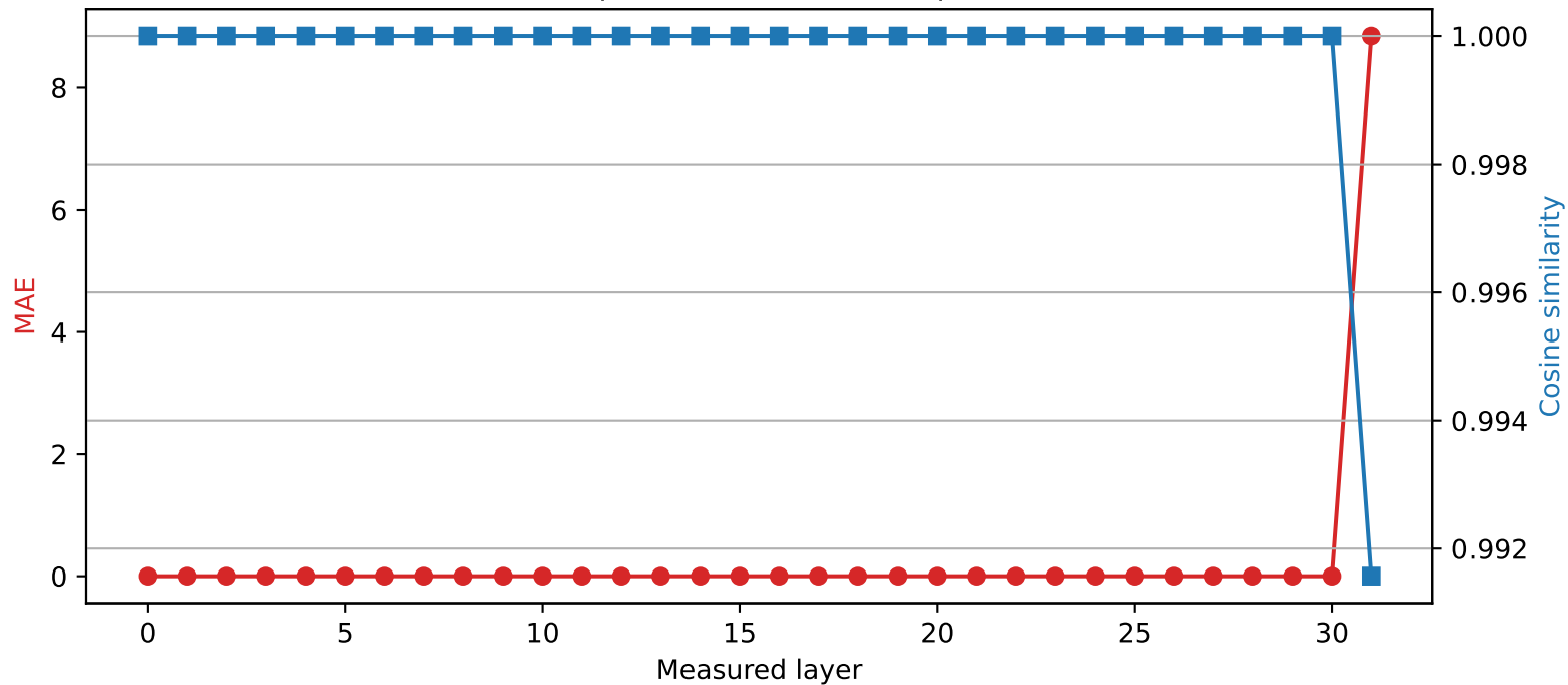
SmolLM2-360M | Quantized layer 30 | float64 \rightarrow int2
