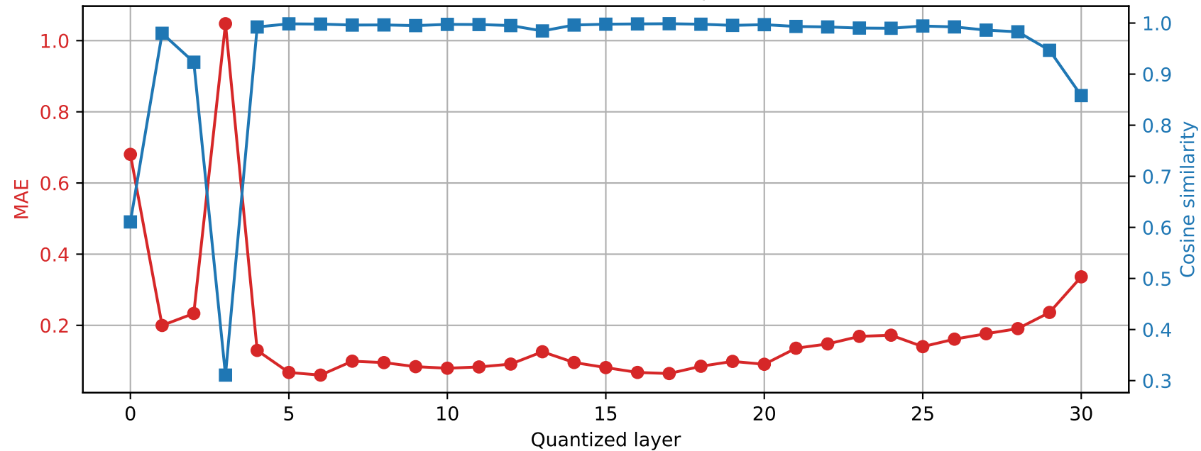
SmolLM2-360M | Prompt 4 Final RMSNorm output damage | float64 → int2
