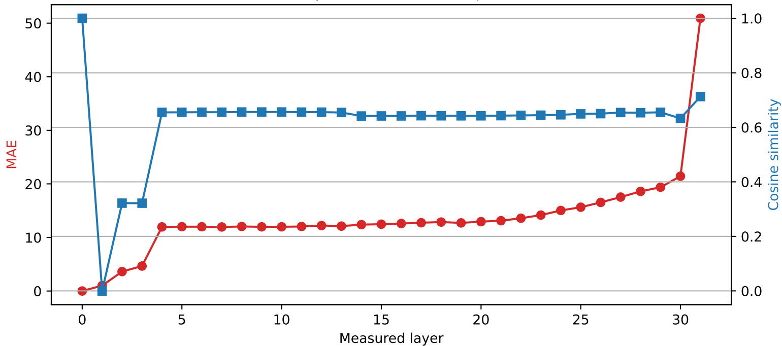
SmolLM2-360M | Quantized layer 0 | float64 → int2
