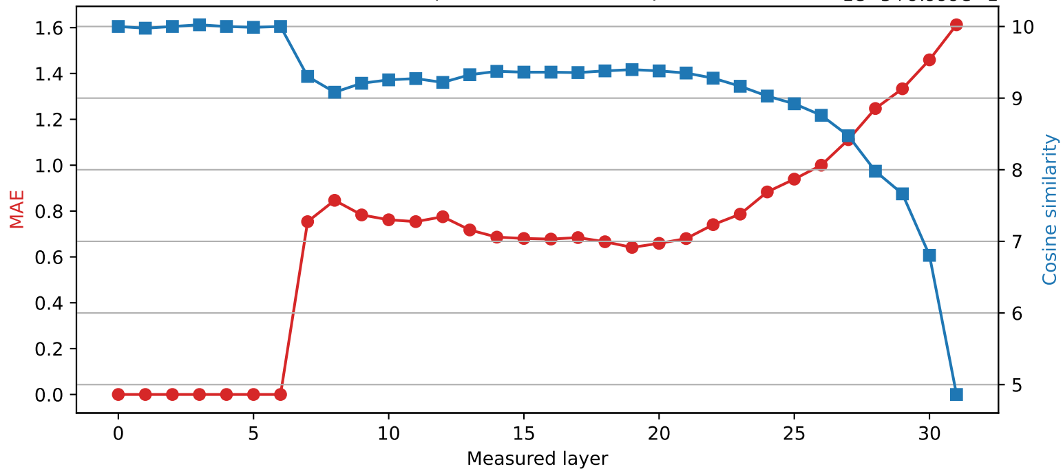
SmolLM2-360M | Quantized layer 6 | float64 → int2
