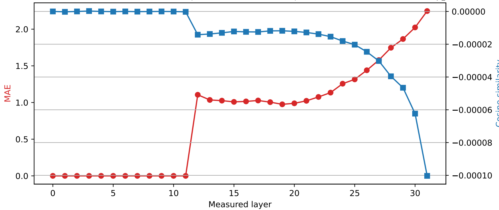
SmolLM2-360M | Quantized layer 11 | float64 → int2
