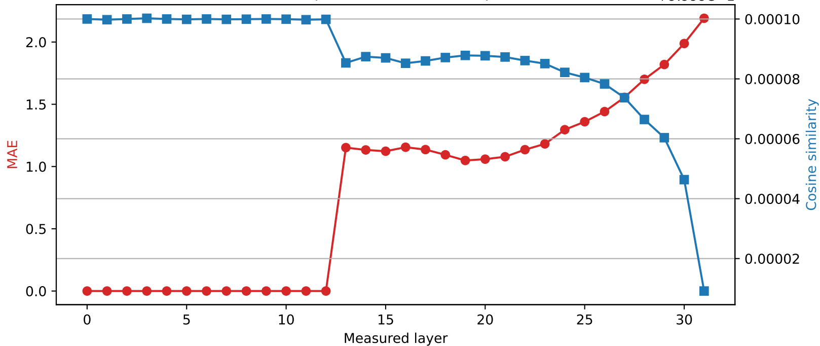
SmolLM2-360M | Quantized layer 12 | float64 → int2
