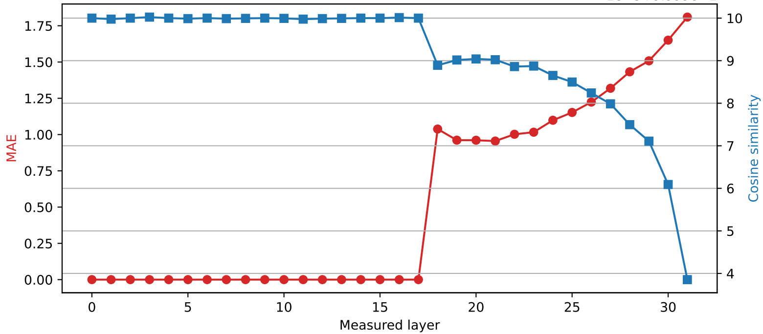
SmolLM2-360M | Quantized layer 17 | float64 \rightarrow int2 1e-5+9.999e-1
