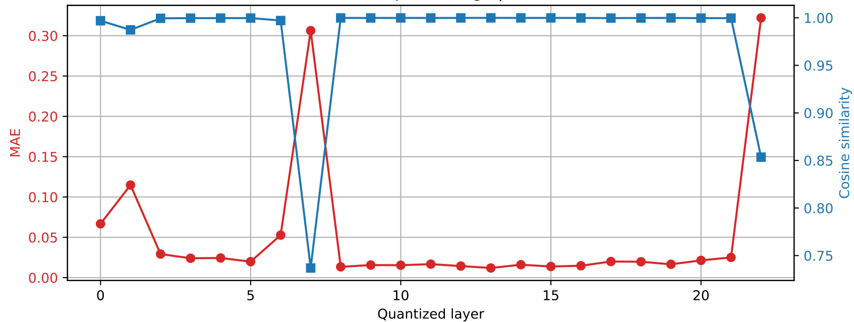
SmolLM2-1.7B-Instruct | Prompt 0 Final RMSNorm output damage | float16 \rightarrow int8
