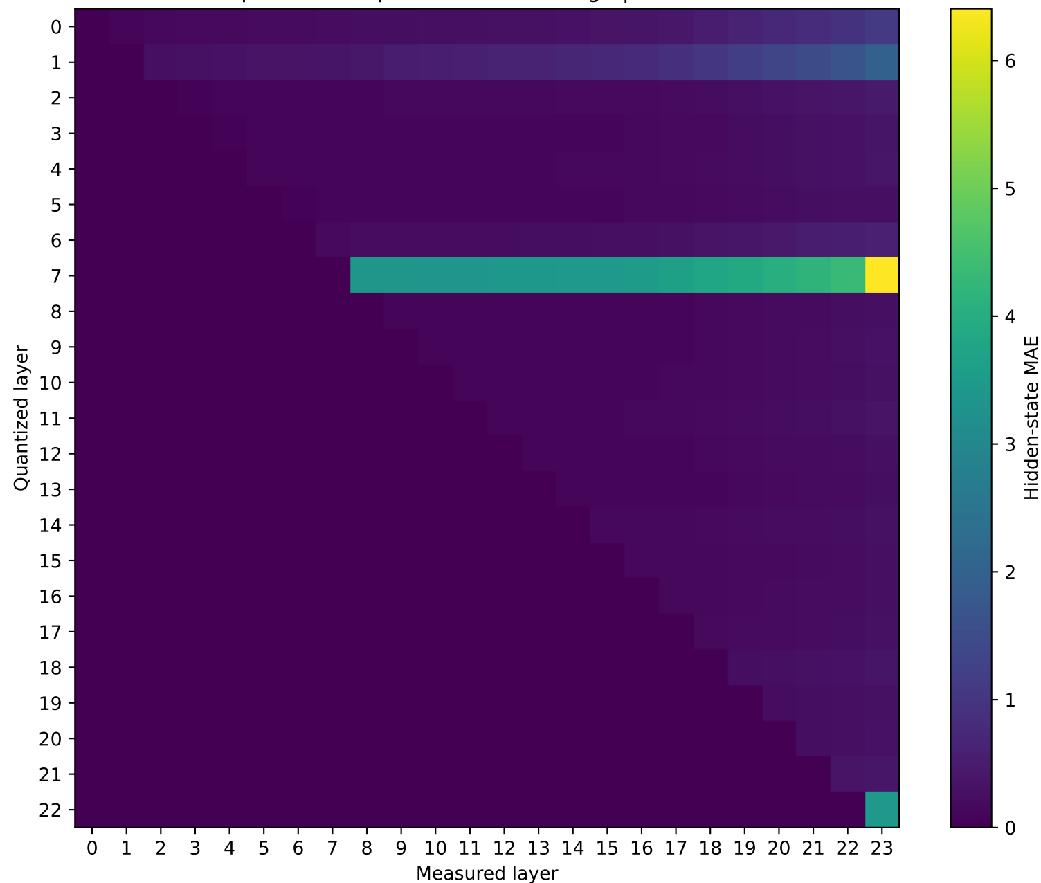
SmolLM2-1.7B-Instruct Prompt 0: MAE representation damage | float16 → int8
