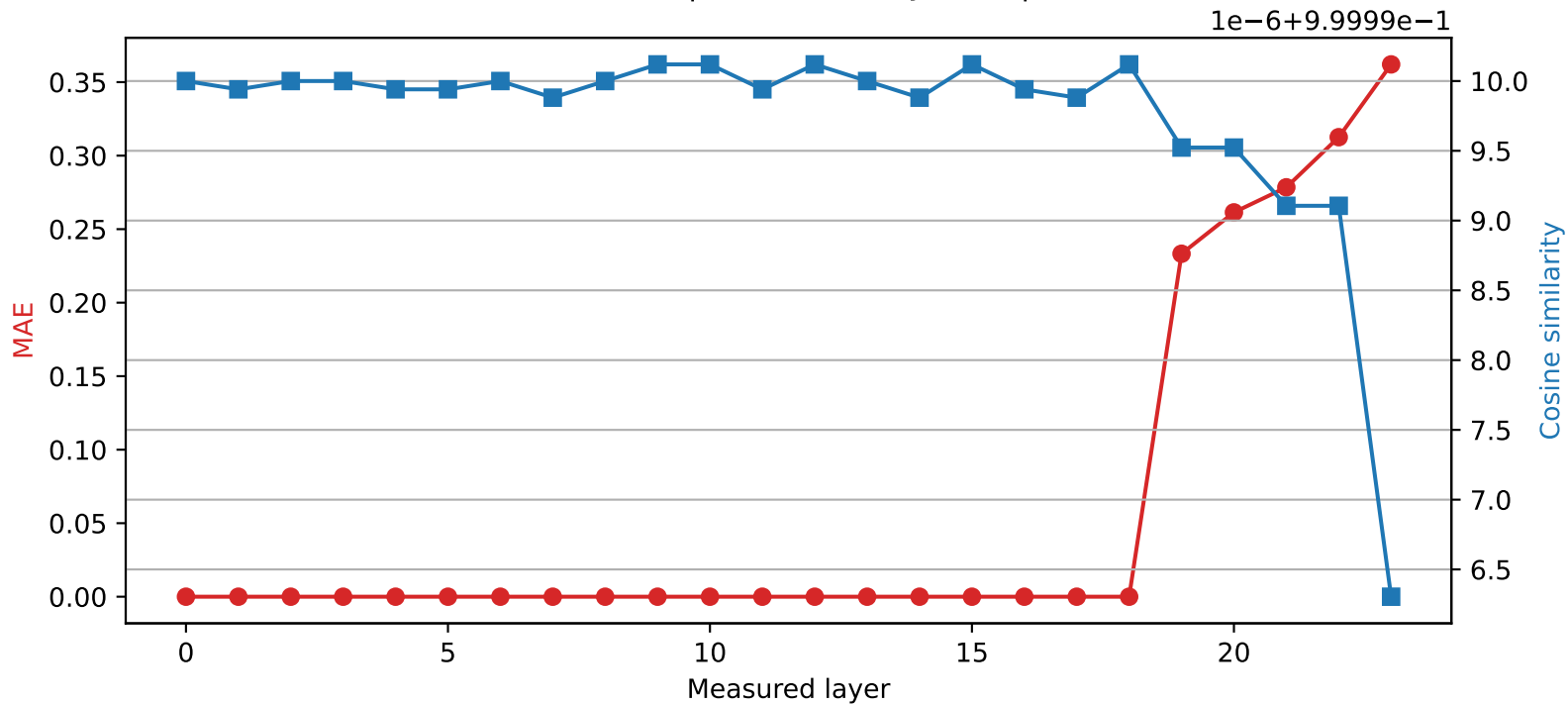
SmolLM2-1.7B-Instruct | Quantized layer 18 | float16 → int8
