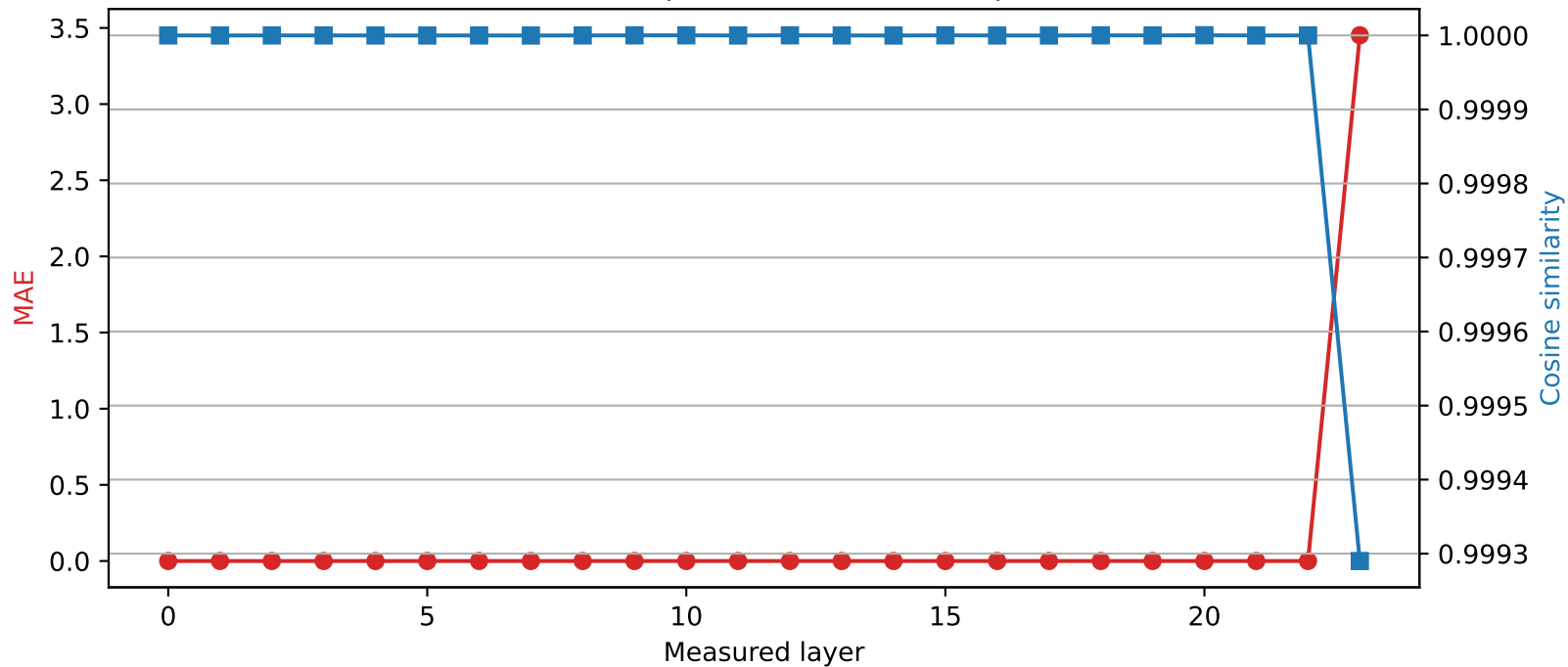
SmolLM2-1.7B-Instruct | Quantized layer 22 | float16 \rightarrow int8
