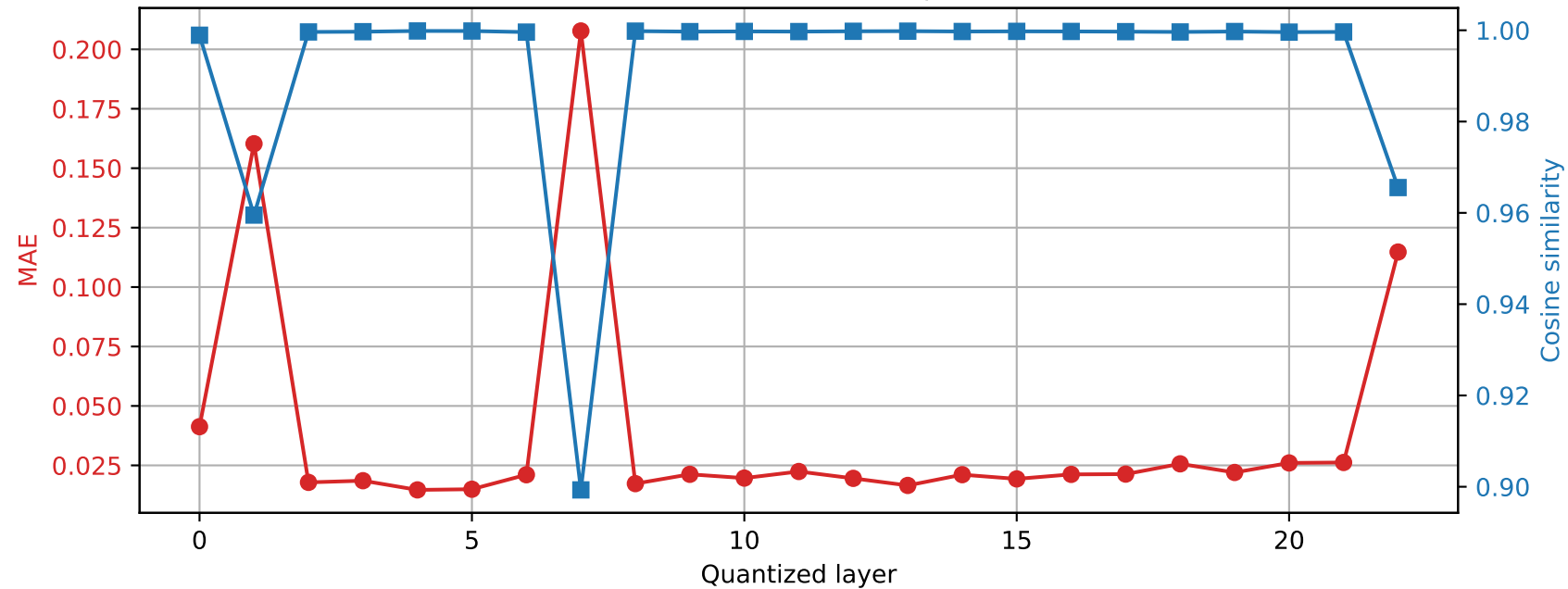
SmolLM2-1.7B-Instruct | Prompt 1 Final RMSNorm output damage | float16 \rightarrow int8
