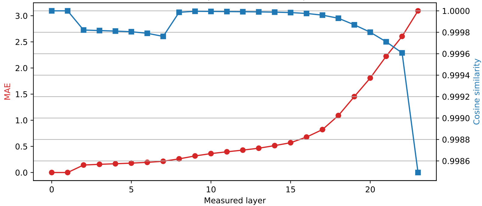
SmolLM2-1.7B-Instruct | Quantized layer 1 | float16 → int8
