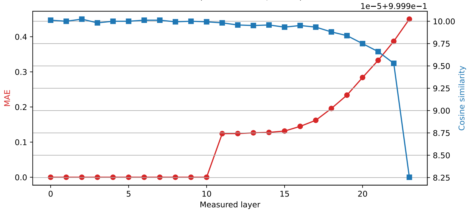
SmolLM2-1.7B-Instruct | Quantized layer 10 | float16 → int8
