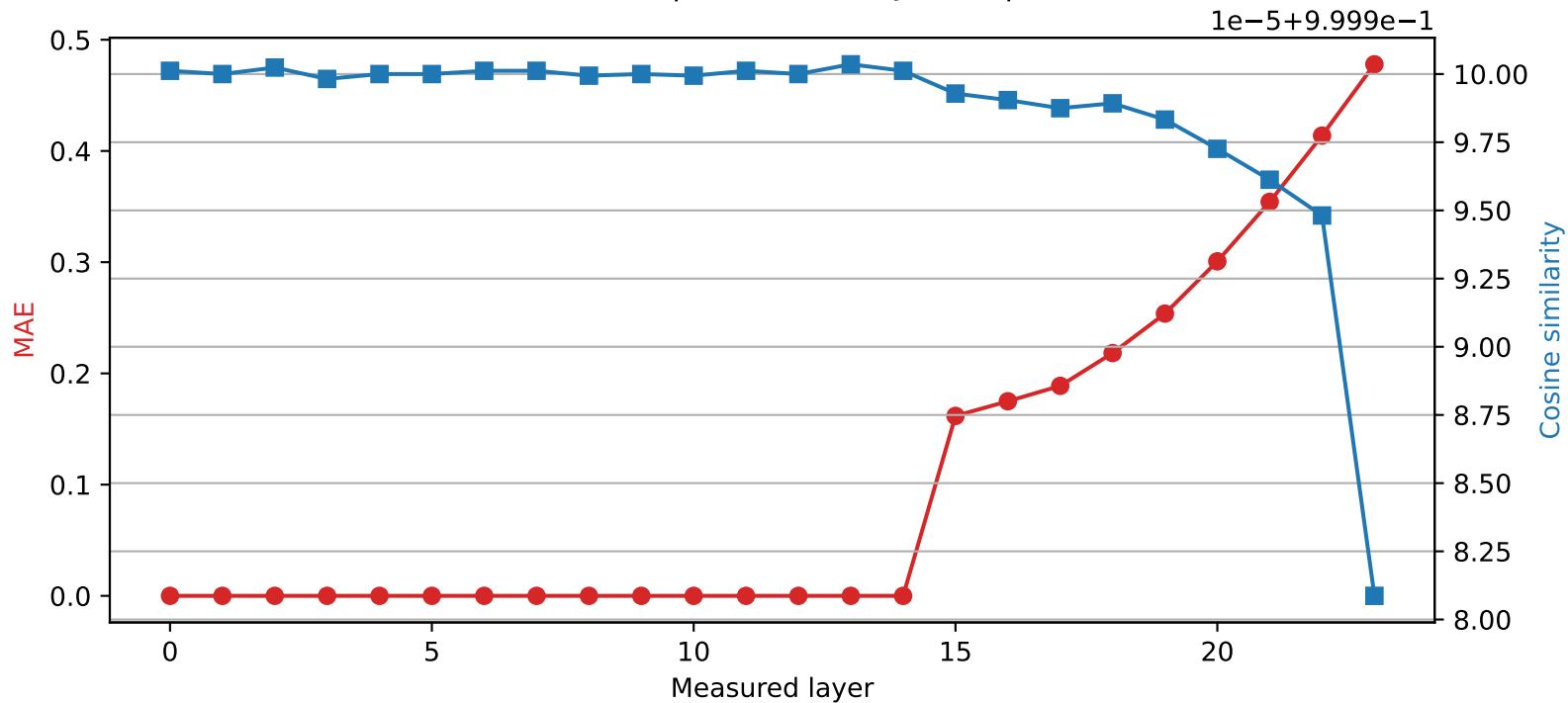
SmolLM2-1.7B-Instruct | Quantized layer 14 | float16 → int8
