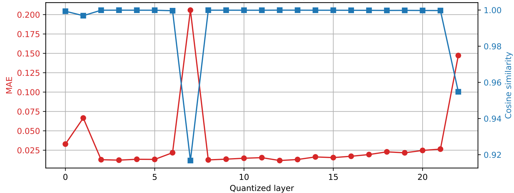
SmolLM2-1.7B-Instruct | Prompt 2 Final RMSNorm output damage | float16 \rightarrow int8
