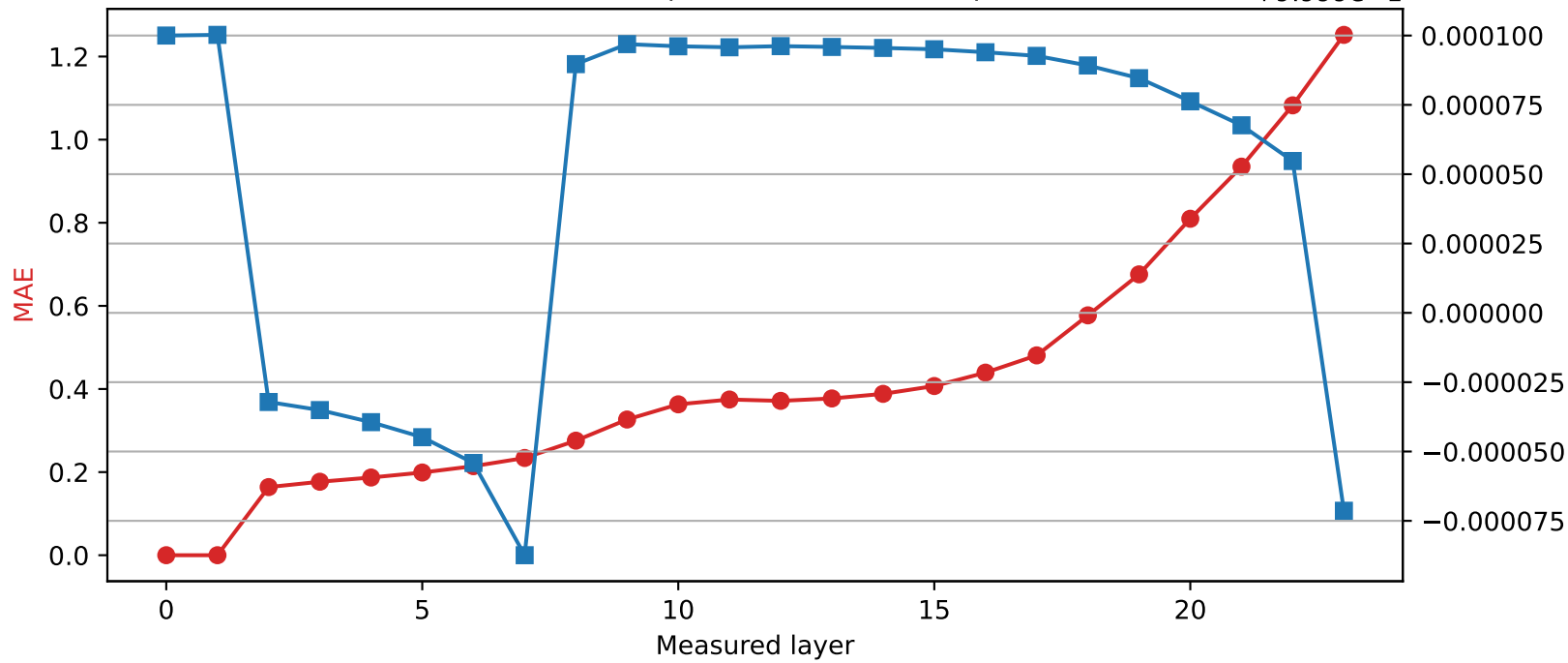
SmolLM2-1.7B-Instruct | Quantized layer 1 | float16 → int8
