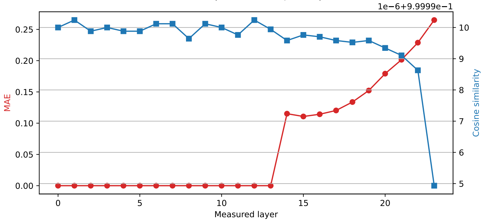
SmolLM2-1.7B-Instruct | Quantized layer 13 | float16 → int8
