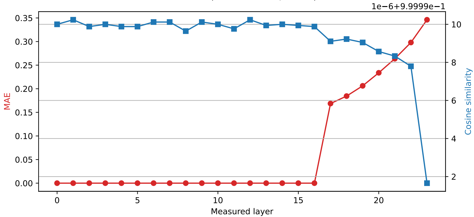
SmolLM2-1.7B-Instruct | Quantized layer 16 | float16 → int8
