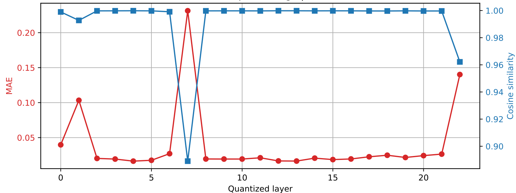
SmolLM2-1.7B-Instruct | Prompt 3 Final RMSNorm output damage | float16 \rightarrow int8
