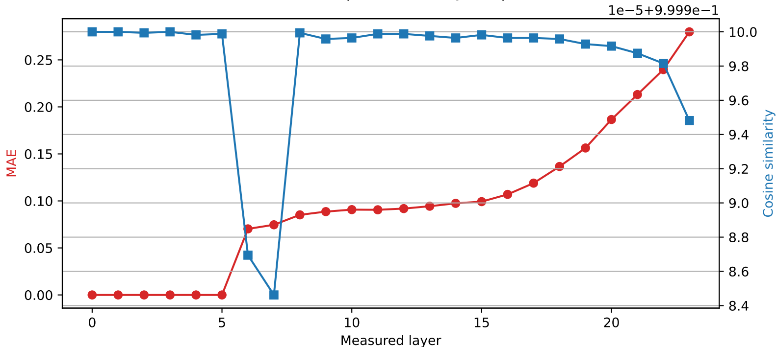
SmolLM2-1.7B-Instruct | Quantized layer 5 | float16 → int8
