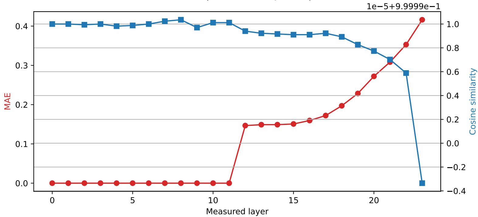
SmolLM2-1.7B-Instruct | Quantized layer 11 | float16 → int8
