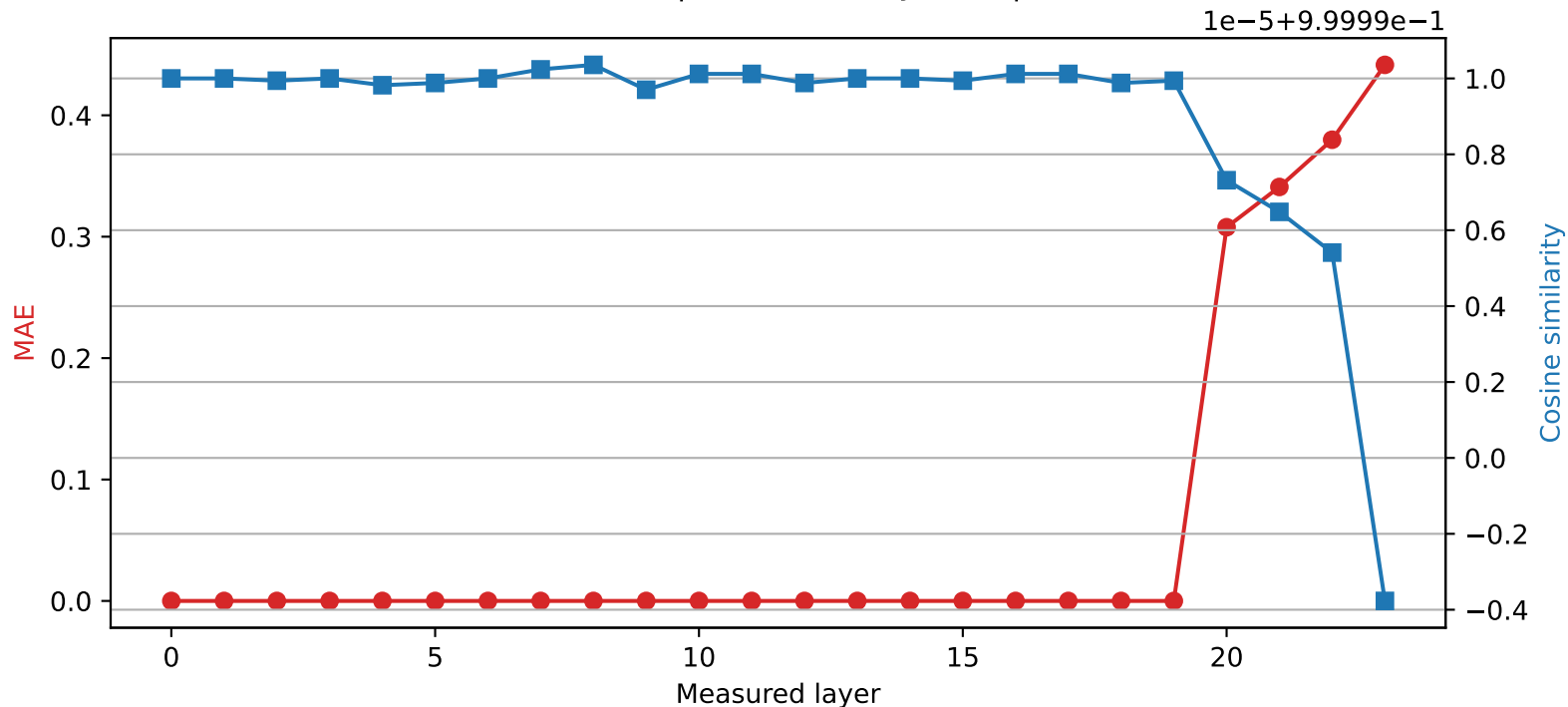
SmolLM2-1.7B-Instruct | Quantized layer 19 | float16 → int8
