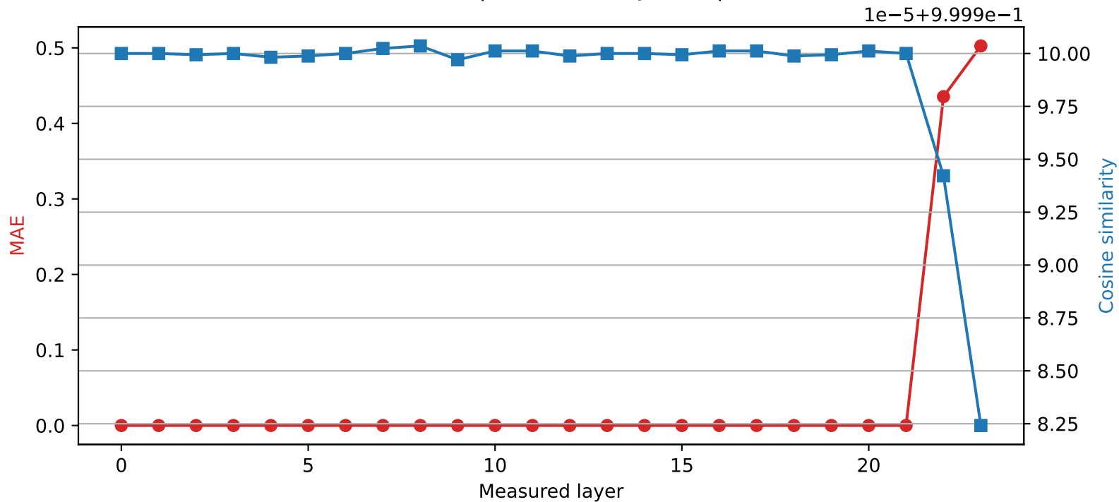
SmolLM2-1.7B-Instruct | Quantized layer 21 | float16 → int8
