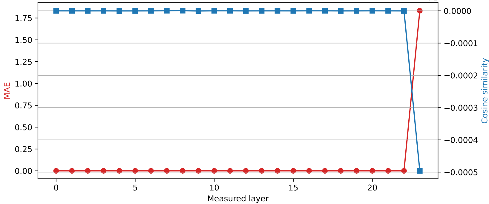
SmolLM2-1.7B-Instruct | Quantized layer 22 | float16 \rightarrow int8
