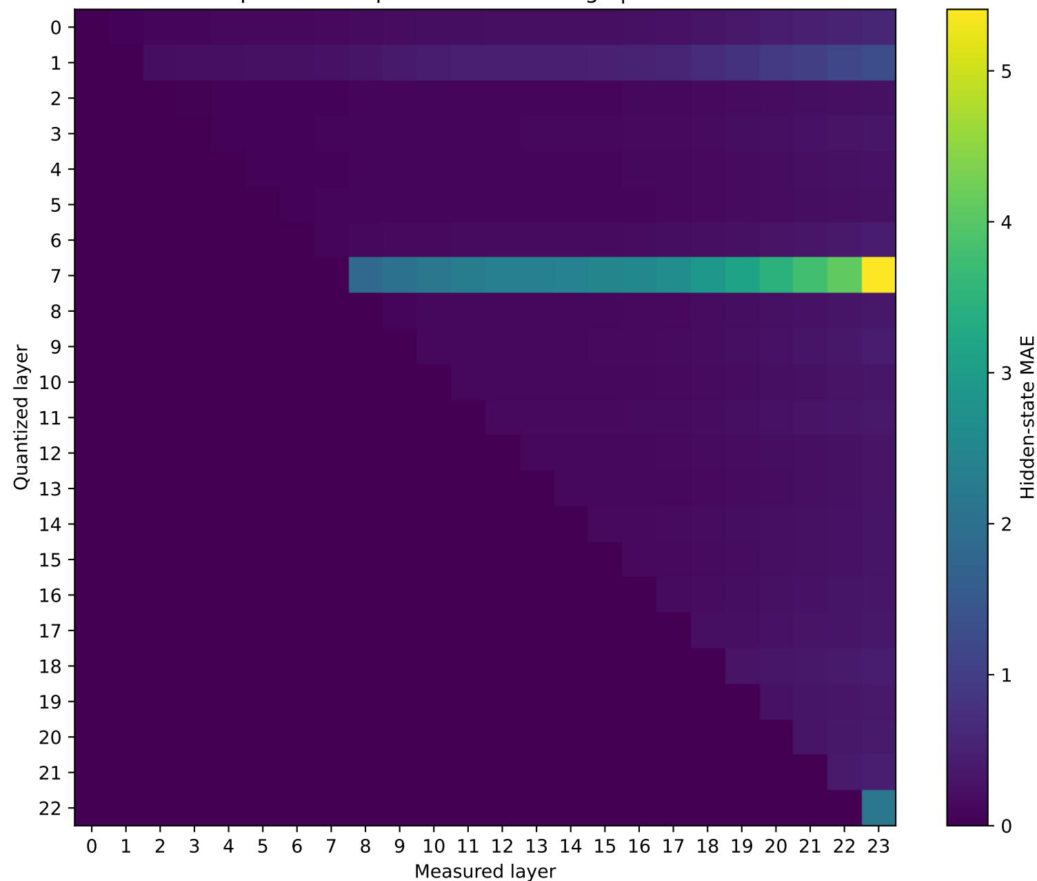
SmolLM2-1.7B-Instruct Prompt 4: MAE representation damage | float16 → int8
