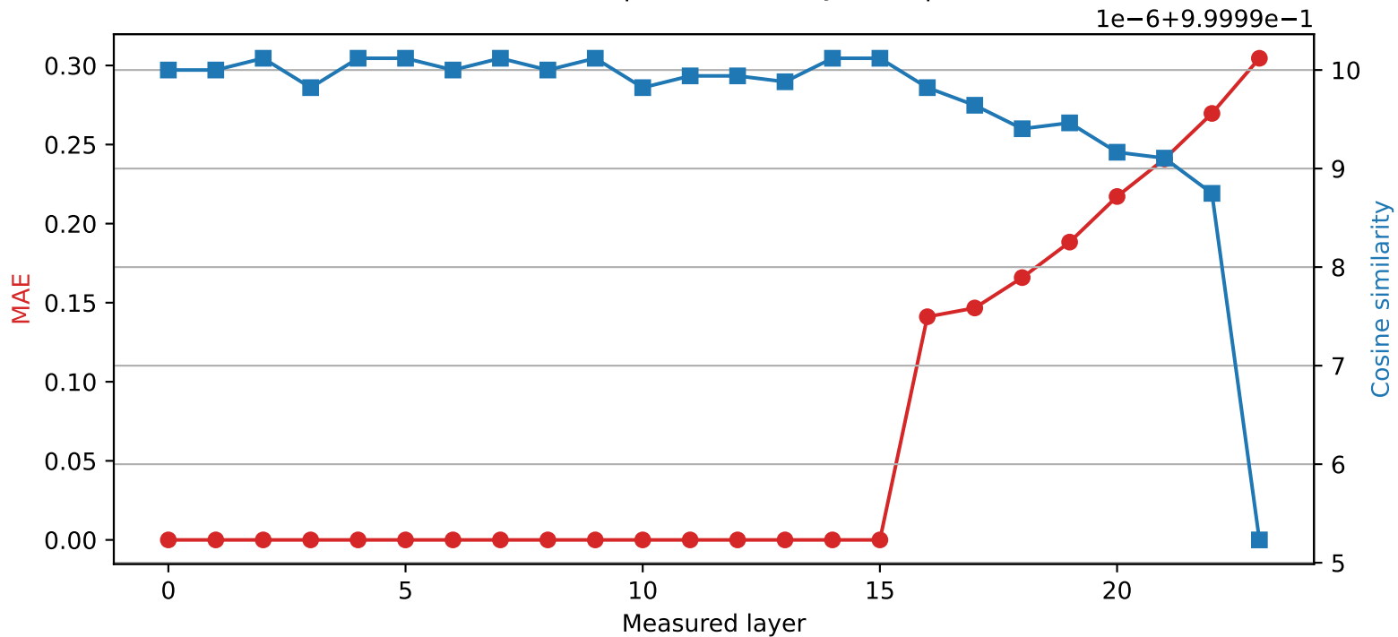
SmolLM2-1.7B-Instruct | Quantized layer 15 | float16 → int8
