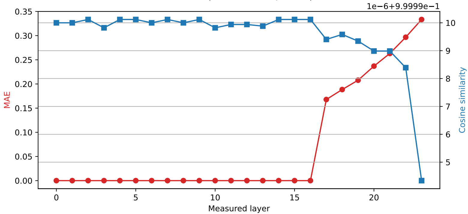
SmolLM2-1.7B-Instruct | Quantized layer 16 | float16 \rightarrow int8
