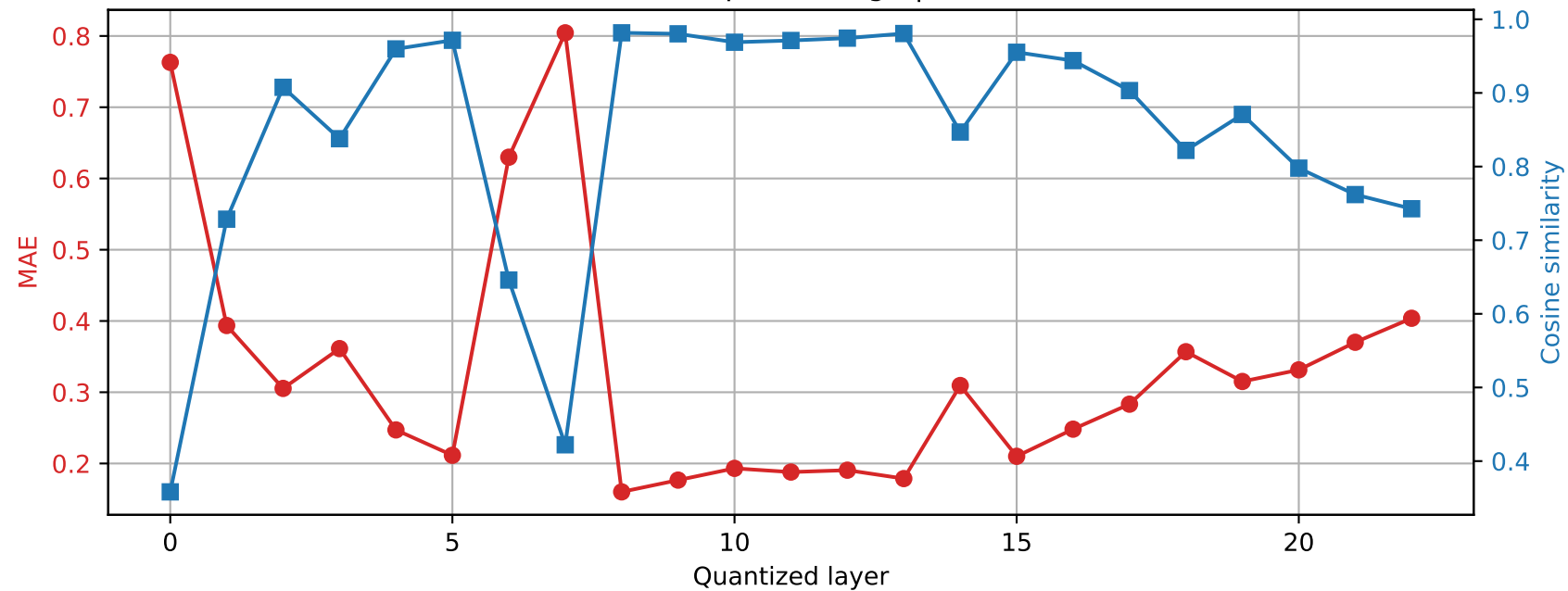
SmolLM2-1.7B-Instruct | Prompt 0 Final RMSNorm output damage | float16 \rightarrow int4
