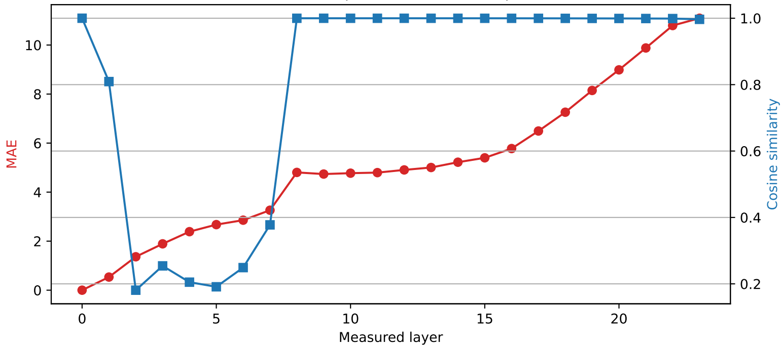
SmolLM2-1.7B-Instruct | Quantized layer 0 | float16 → int4
