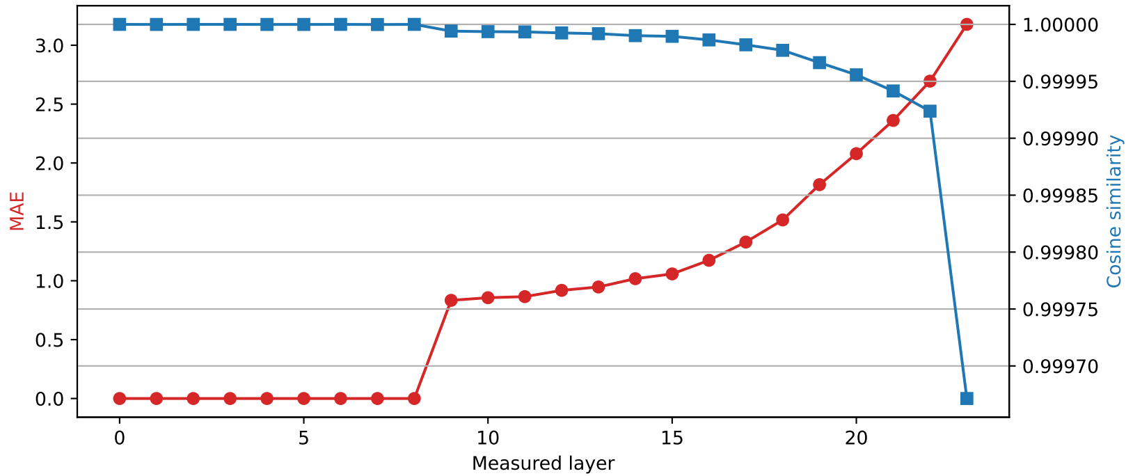
SmolLM2-1.7B-Instruct | Quantized layer 8 | float16 → int4
